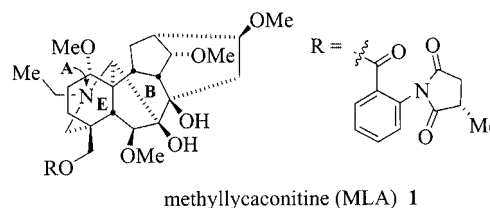
Figure 1. Structure of the alkaloid methyllycaconitine (MLA) illustrating the ABE rings.
