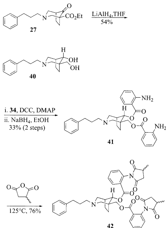
Scheme 5.
