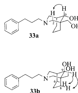
Figure 2. NOE effects observed for the diastereomers 33a and 33b . In the case of compound 33a , no interactions were detected between 9-H and 6-H ax or 8-H ax , while compound 33b showed no NOE between 9-H and 2-H ax .
